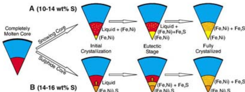
Fig. 3. Cross section through Mars, illustrating two possible crystallization regimes for the martian core. Solid (Fe,Ni), yellow; solid \text{Fe}_3\text{S} , orange; liquid sulfide, red; mantle, blue; crust, black (not drawn to scale). (A) Snowing-core hypothesis. (B) Sulfide inner-core hypothesis.
